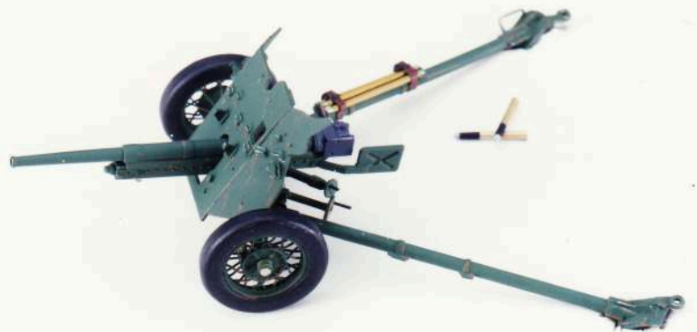
RUSSIAN 45mm ANTI-TANK GUN Model 1937 A.M.F.A. 98 E1-55
