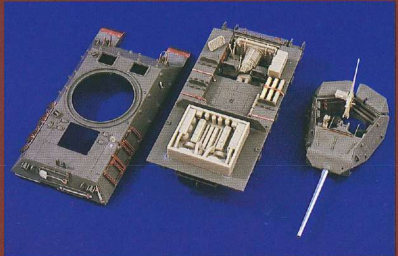
1584 M10 Tank Destroyer Detail Set 1:35
