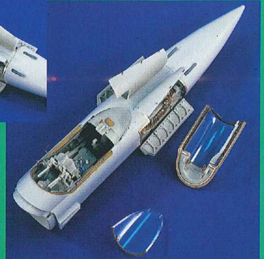
N°1739 F5E Tiger Detail Set + full Cockpit (Hasegawa) 1:32
