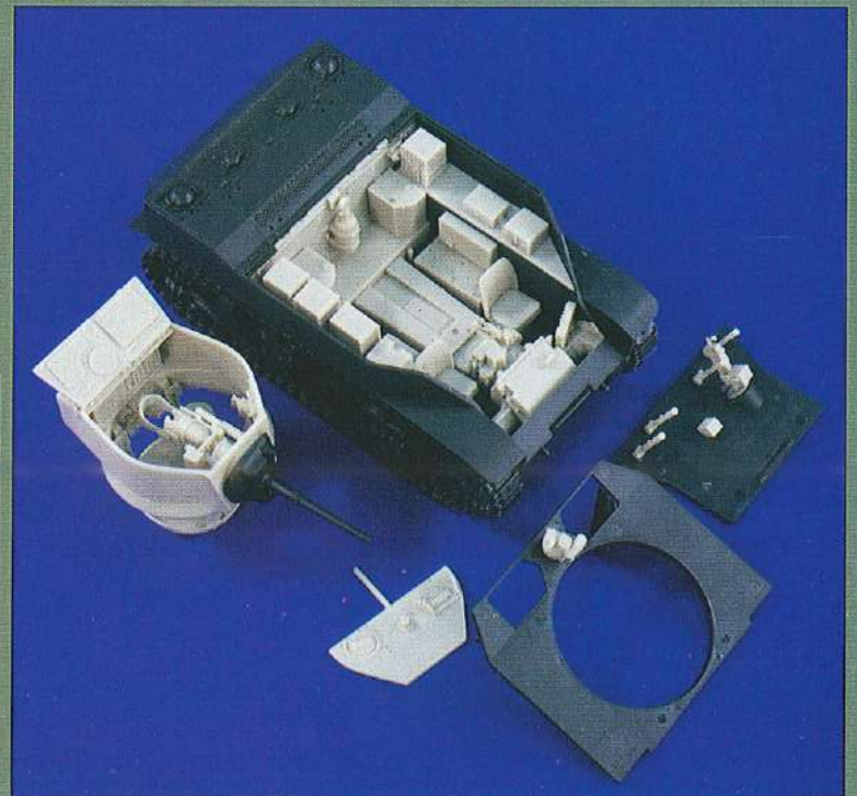
1562 M5 A1 Stuart Interior (for Tamiya) 1:35 Scale
