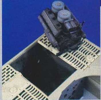
N°1019 Tiger I Engine & Compartment 1:15
