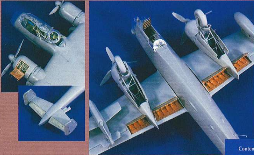
1659 Dornier 217-E5 Detail Set 1:48 (for Revell-Monogram)
