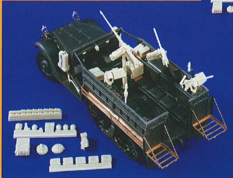
1610 M3 Halftrack Detail Set 1:35
