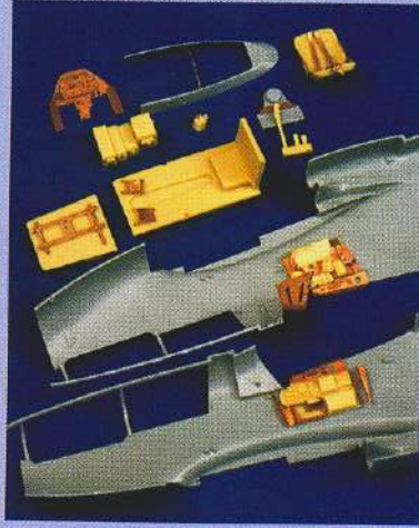
N°0787 P-51 Mustang Cockpit Detail Set (Hasegawa) 1:32
