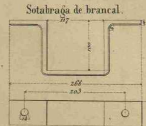
Sotabraja de brancal.
