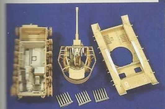
N°1534 Panzer IV Interior (Tamiya) 1:35
