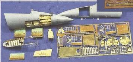
N°0447 F-15C Eagle Super Detail Set (Hasegawa) 1:48
