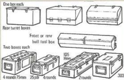
N°0346 Tank Tool & Equipment Boxes 1:35
